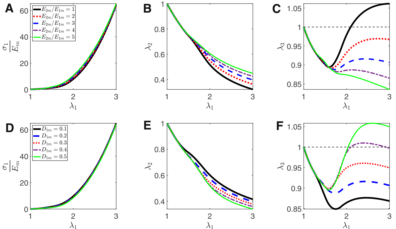
Fig. 6. The influence of matrix stiffening and transition strain on the stress (A, D), in-plane transverse stretch (B, E), and auxetic behaviour (C, F). Reference parameters D_{1f} = 0.2, D_{2f} = 0.4, E_{1f}/E_{1m} = 1.5, \theta = 45^\circ, E_{2f}/E_{1m} = 8, D_{1m} = 0.2, D_{2m} = D_{1m} + 0.2, E_{2m}/E_{1m} = 3, K/E_{1m} = 30 have been used.
