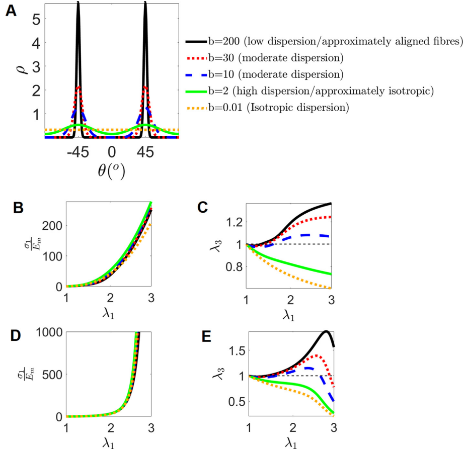
Fig. 9. Effects of fibre dispersion on the stress-stretch curve and auxetic behaviour, for bilinear (B,C) and exponential (D,E) fibre models with neo-Hookean model for the matrix. The probability density function, \rho , for the fibres dispersion around the mean fibre directions ( \theta = \pm 45^\circ ) is also shown in (A).
