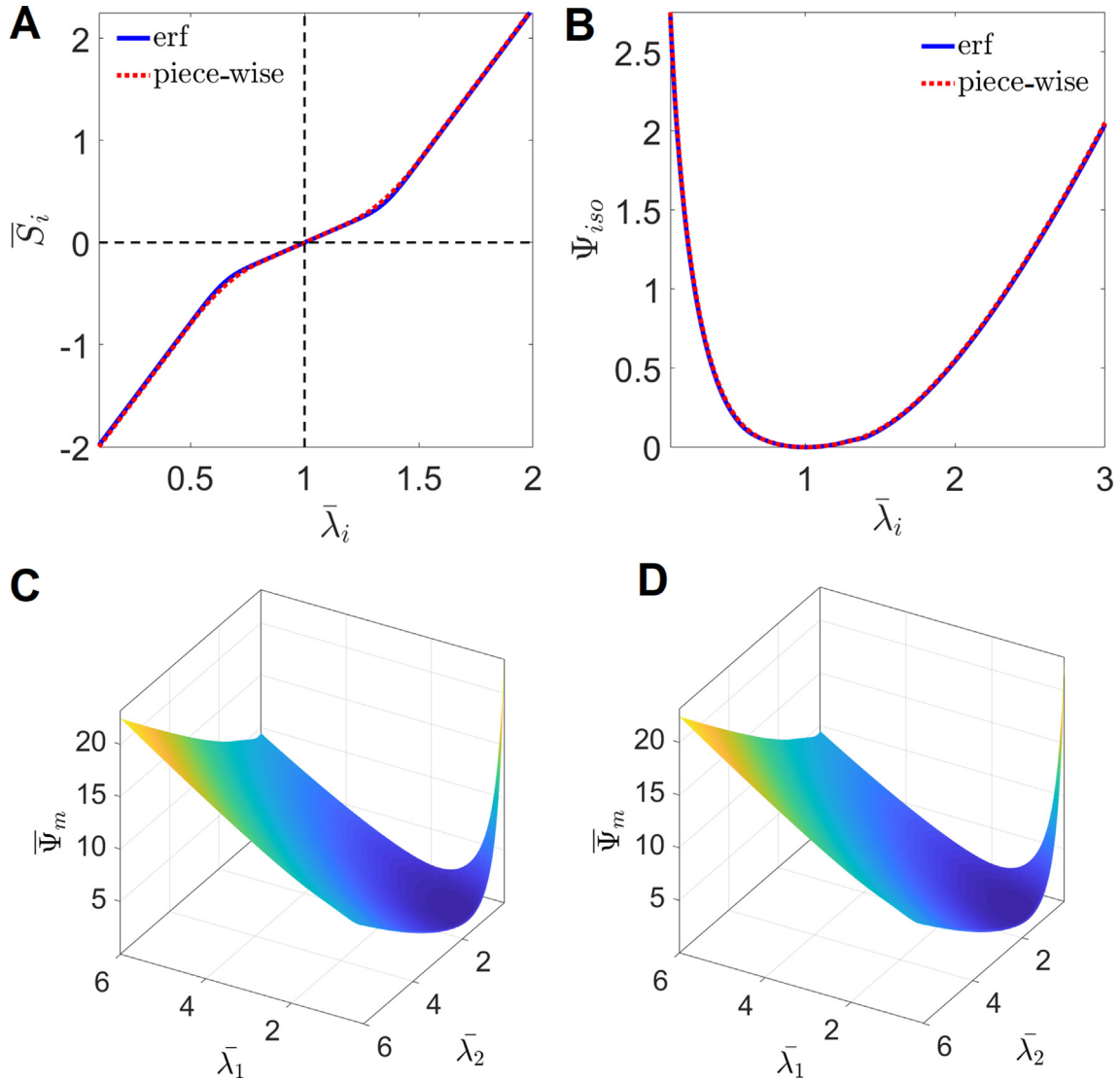
Fig. A1. Comparison of the two proposed strain-stiffening models for matrix in tension and compression; (A) Stress-stretch, (B) strain energy density function, (C) the strain energy density surface for the error function formulation (Eq. (A.11)), and (D) the strain energy density surface for the piece-wise formulation (Eq. (14)). The material parameters of D_{1m} = 0.2, D_{2m} = 0.5, E_{1m} = 1, E_{2m} = 3, and \beta_m = 5 have been used.
