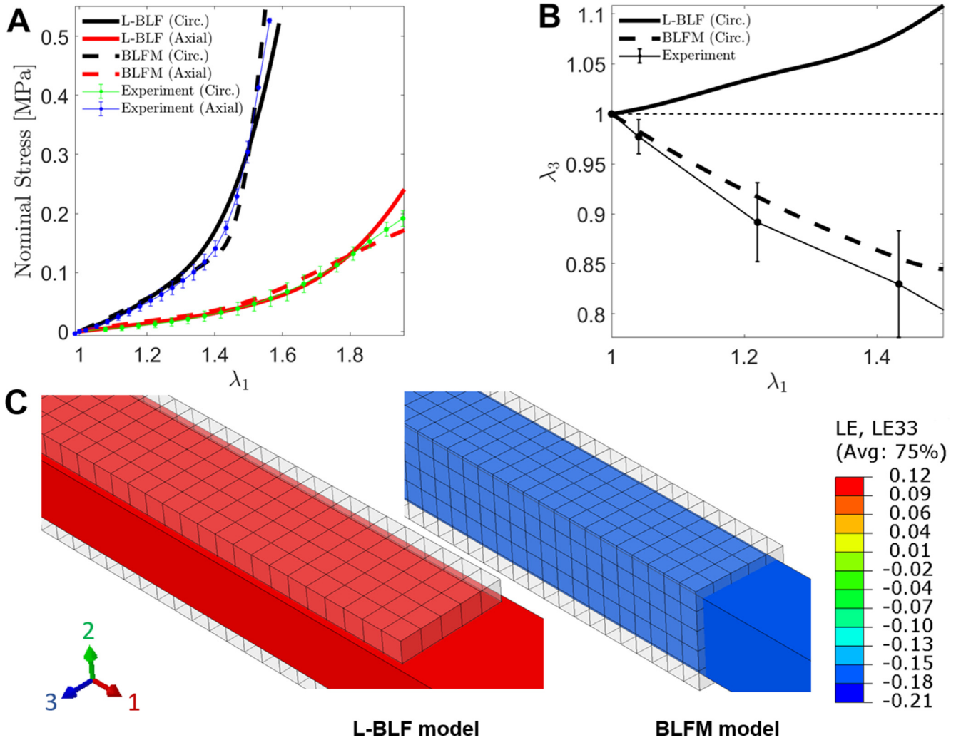
Fig. 7. The capability of the BLFM model to reproduce the stress-stretch experimental data of the uniaxial tension of ascending aorta FitzGibbon and McGarry (2020) (A) and out-of-plane stretch in circumferential test (B). FE results of the uniaxial tension tests for BLFM model and L-BLF models are also shown (C). "L-BLF" stands for a linear matrix model in parallel with the BLF model.
