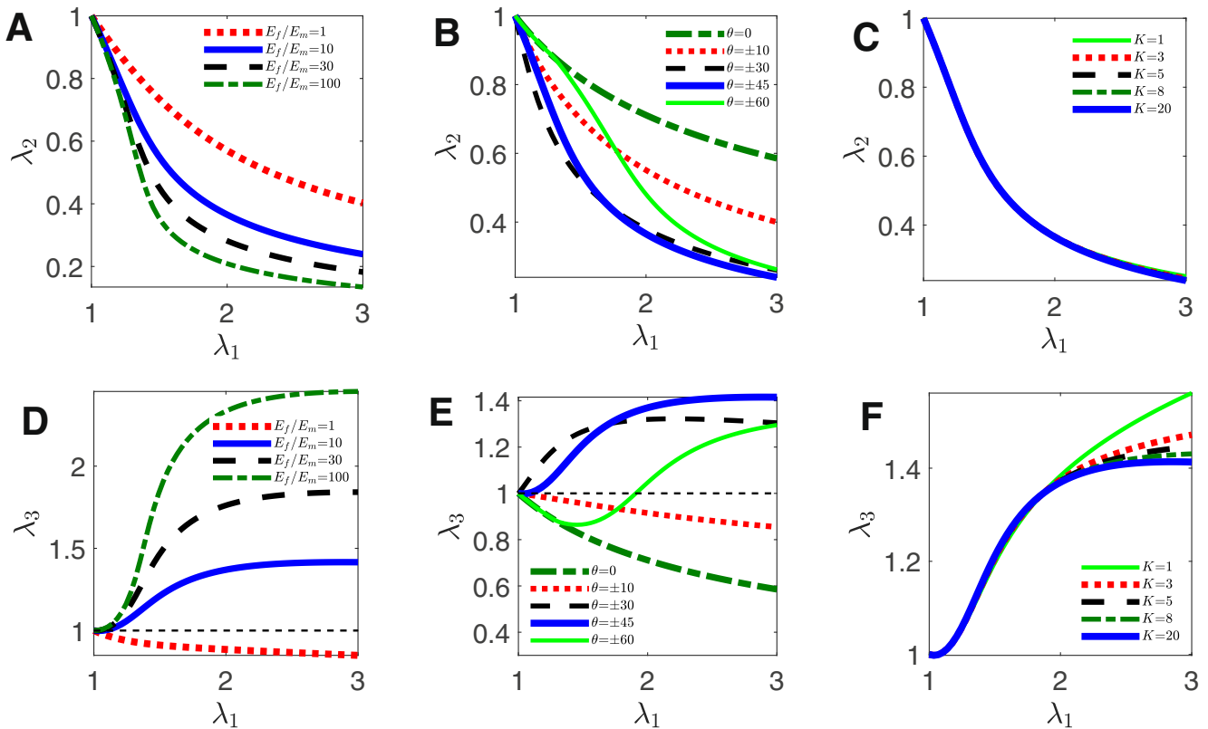
Fig. 3. Influence of the fibre to matrix stiffness ratio (A, D), fibre angle (B, E) and compressibility (C, F) on the in-plane (first row) and out-of-plane stretch \lambda_3 (Second row) for the uniaxial extension of a cubic element of fibrous materials. A neo-Hookean matrix with a linear fibre model with the reference parameters value of \theta = \pm 45^\circ , E_m = 0.5 , E_f/E_m = 10 and K/\mu = 100 have been used in all plots. \lambda_1 is the stretch in the loading direction.
