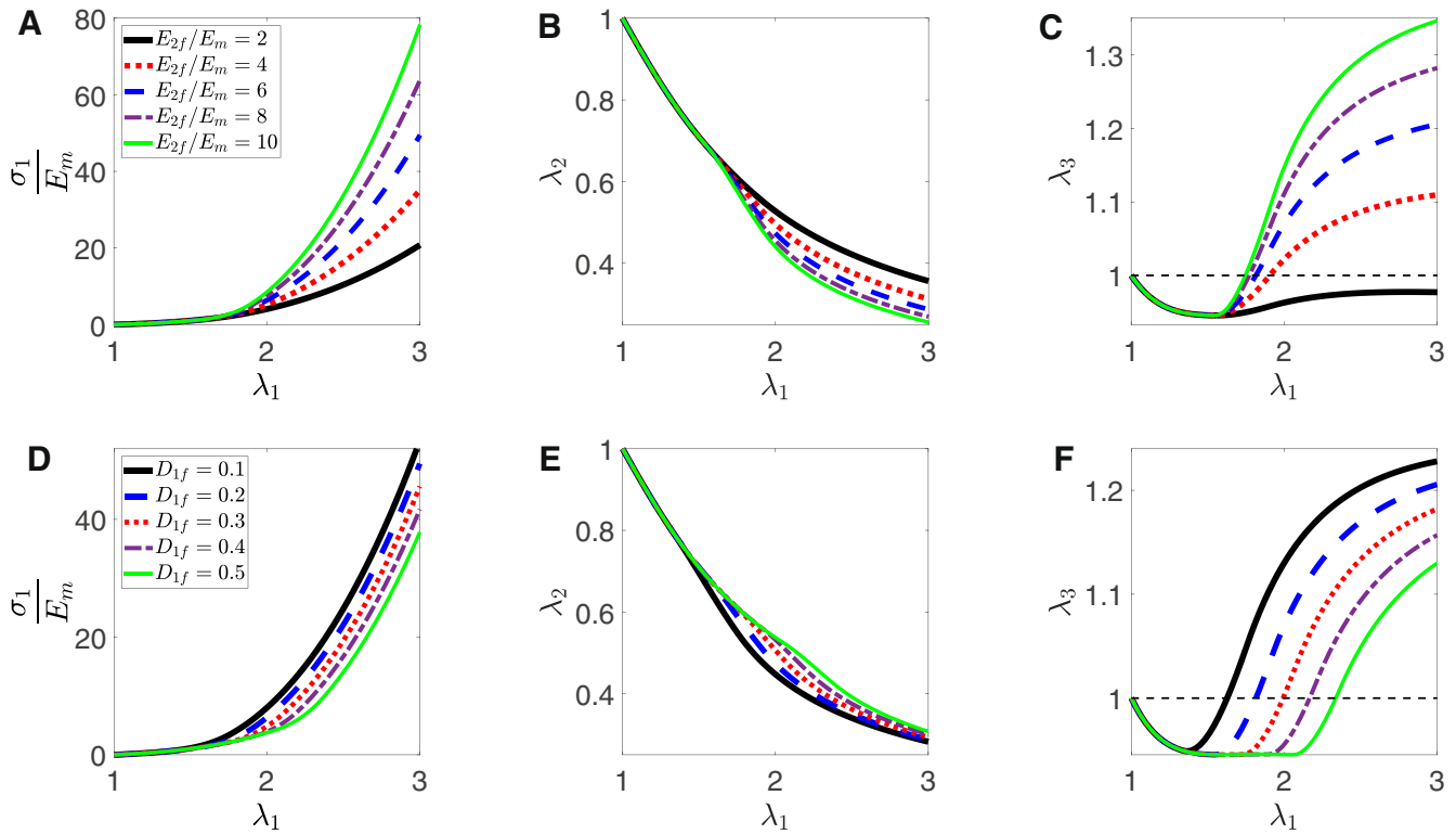
Fig. 5. The influence of fibre strain-stiffening and transition strain on the stress (A, D), in-plane transverse stretch (B, E) and out-of-plane stretch (C, F). Reference parameters E_{1f}/E_m = 1.5, \theta = 45^\circ, E_{2f}/E_m = 6, D_{1f} = 0.2, D_{2f} = D_{1f} + 0.2 have been used.
