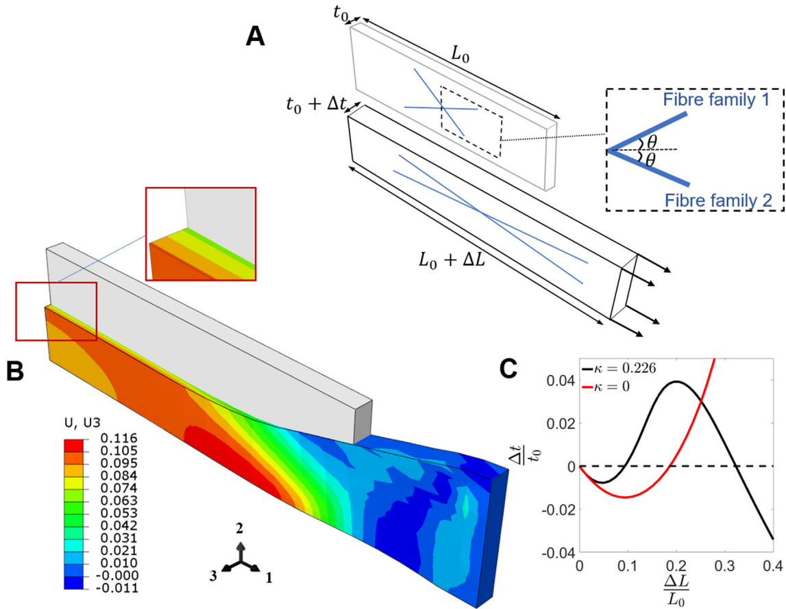
Fig. 1. Results of the Abaqus Benchmark Guide example Abaqus (2017) for uniaxial tension of an adventitial strip cut along the circumferential direction. (A) Two fibre families oriented as \theta = \pm 49.98^\circ are considered. (B) Increase in the thickness of the strip in case of fully aligned fibres ( \kappa = 0 ) at \frac{\Delta L}{L_0} = 0.33 . (C) An increase in the thickness of the strip is computed for \frac{\Delta L}{L_0} > 0.2 in the case of fully aligned fibres ( \kappa = 0 ) and for 0.09 < \frac{\Delta L}{L_0} < 0.3 in the case of dispersed fibres ( \kappa = 0.226 ). The reader is refer to Abaqus (2017) for details of material parameters and dimensions.
