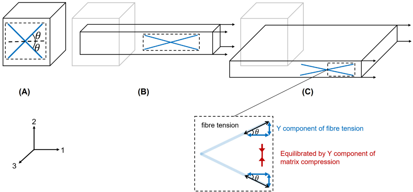
Fig. 2. Schematic of the uniaxial tension of a fibre-reinforced cube with two fibre families. (a) undeformed cube (b) deformed cube without auxetic behaviour, and (c) deformed cube with auxetic behaviour. The fibres are distributed in (1–2) plane.
