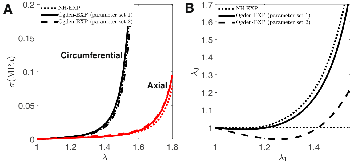
Fig. 8. Comparison of Ogden and neo-Hookean matrix in parallel with the exponential fibre model. The combination of Ogden with exponential fibre model postpones the development of auxetic behaviour in comparison to the neo-Hookean matrix with exponential fibre model (B) while the stress-stretch curves are the same for both models (A). The parameters \mu = 0.0014 MPa, k_1 = 0.0051 MPa and k_2 = 15.4 have been used for NH-Exp model and two parameter sets (i.e., set 1: \mu_1 = \mu_2 = 0.0014 MPa, \alpha_1 = -\alpha_2 = 1.5 , k_1 = 0.0051 MPa, k_2 = 15.4 and set 2: \mu_1 = \mu_2 = 0.0024 MPa, \alpha_1 = -\alpha_2 = 4 , k_1 = 0.0015 MPa, k_2 = 15.4 ) have been used for Ogden-Exp model.
