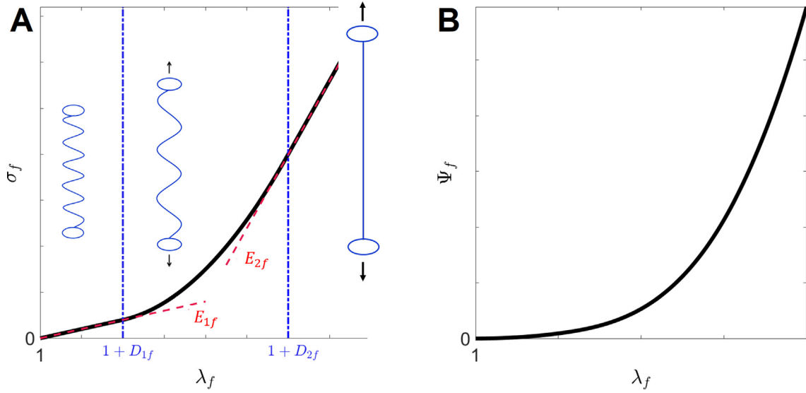
Fig. 4. A schematic illustration of a typical \sigma_f - \lambda_f (A) and \Psi_f - \lambda_f (B) curves for the proposed BLF model. The nature of the parameters E_{1f}, D_{1f}, E_{2f} and D_{2f} , and the uncoiling of the collagen fibres during each deformation regime are illustrated. D_{1f} is the nominal strain at the end of the first linear regime which is controlled by the initial slope E_{1f} . D_{2f} is the nominal strain at the beginning of the second linear regime which is controlled by the slope E_{2f} . The low-stiffness and the high-stiffness linear regime are connected by a transition regime between D_{1f} and D_{2f} .
